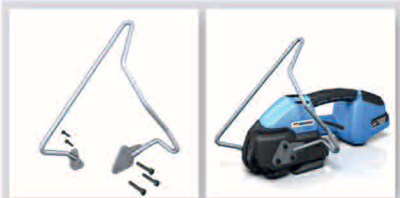
Suspension bow for stationary application
